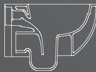
CLEAN FLUSH HUNG WC Art. 5520/CL - Pag. 16
