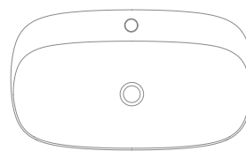
Art. 5512 - 72 x 42 x h6 cm / total 18 cm MOON 70A
